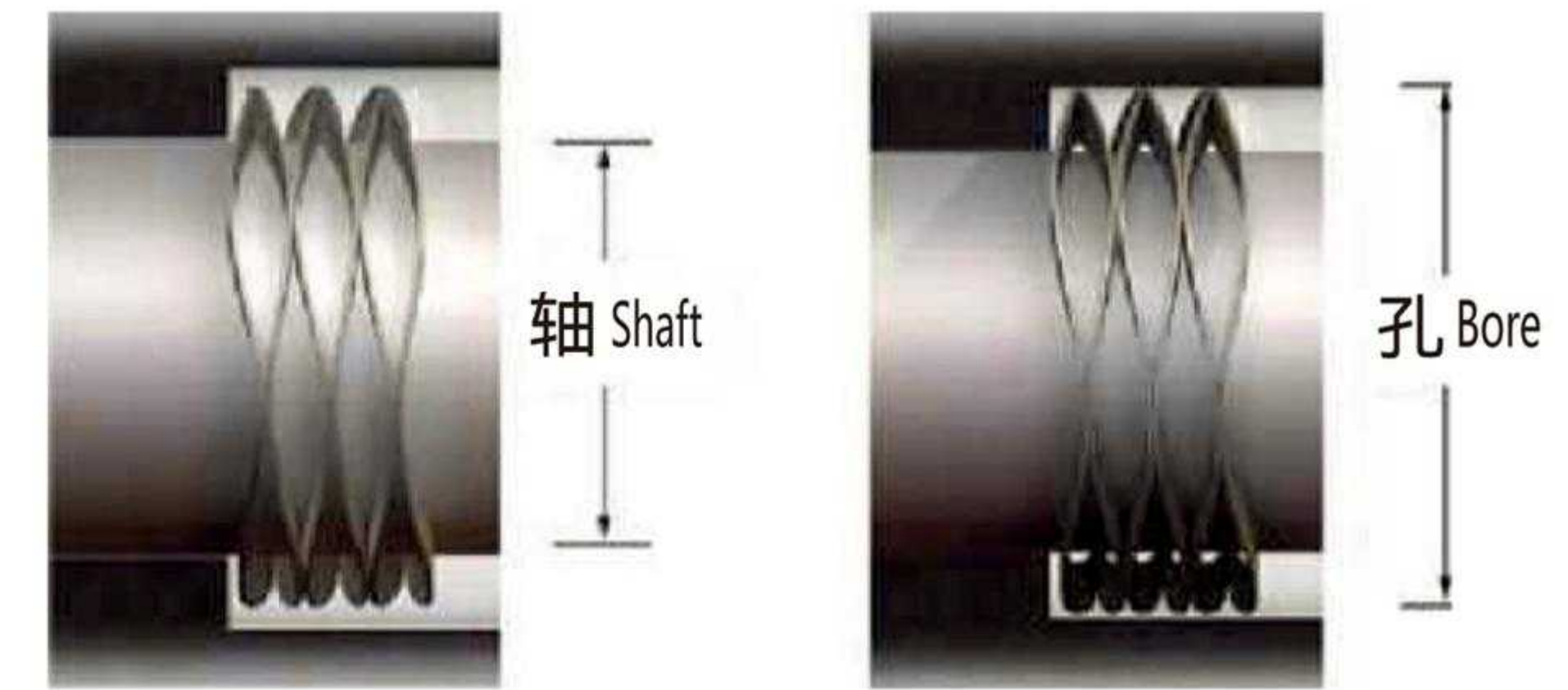
轴引导(内径靠近轴) Shaft Pilot
